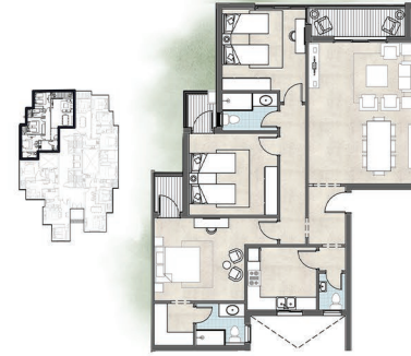
Dejoja Residences Type -B Ground Floor Plan GROSS AREA= 177 SQ.METER
